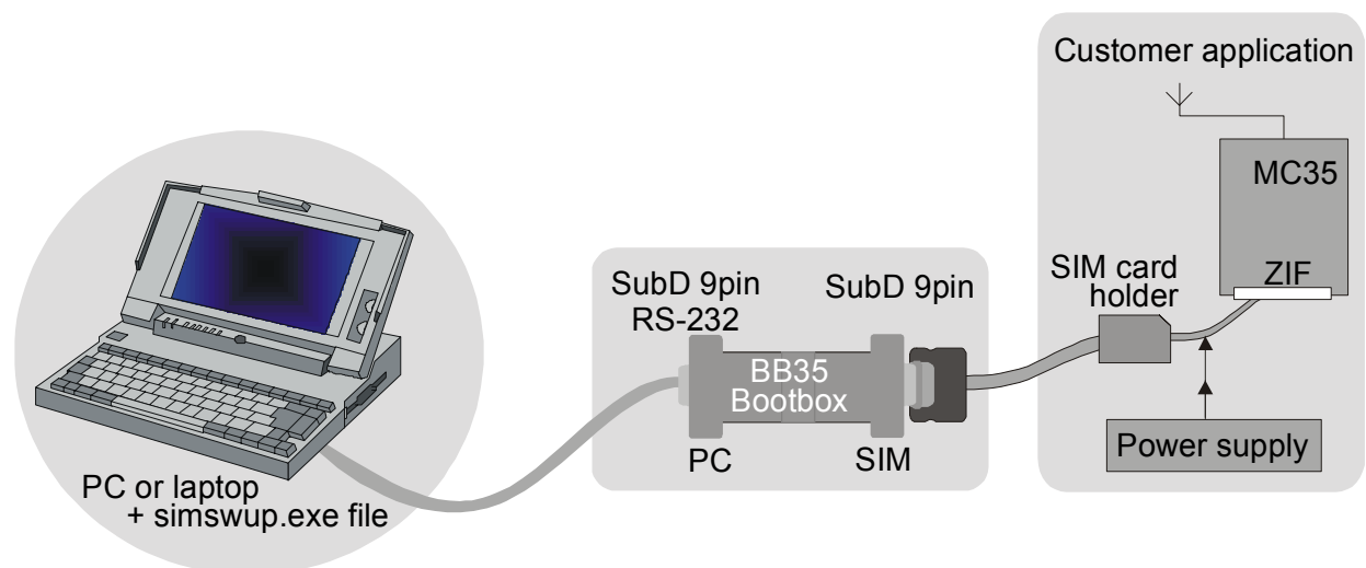
Figure 18: Connecting the BB35 Bootbox to your MC35 application platform
