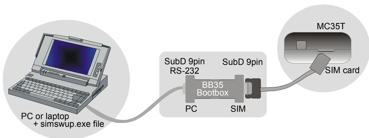
Figure 17: Connecting the BB35 Bootbox to the MC35 Terminal
