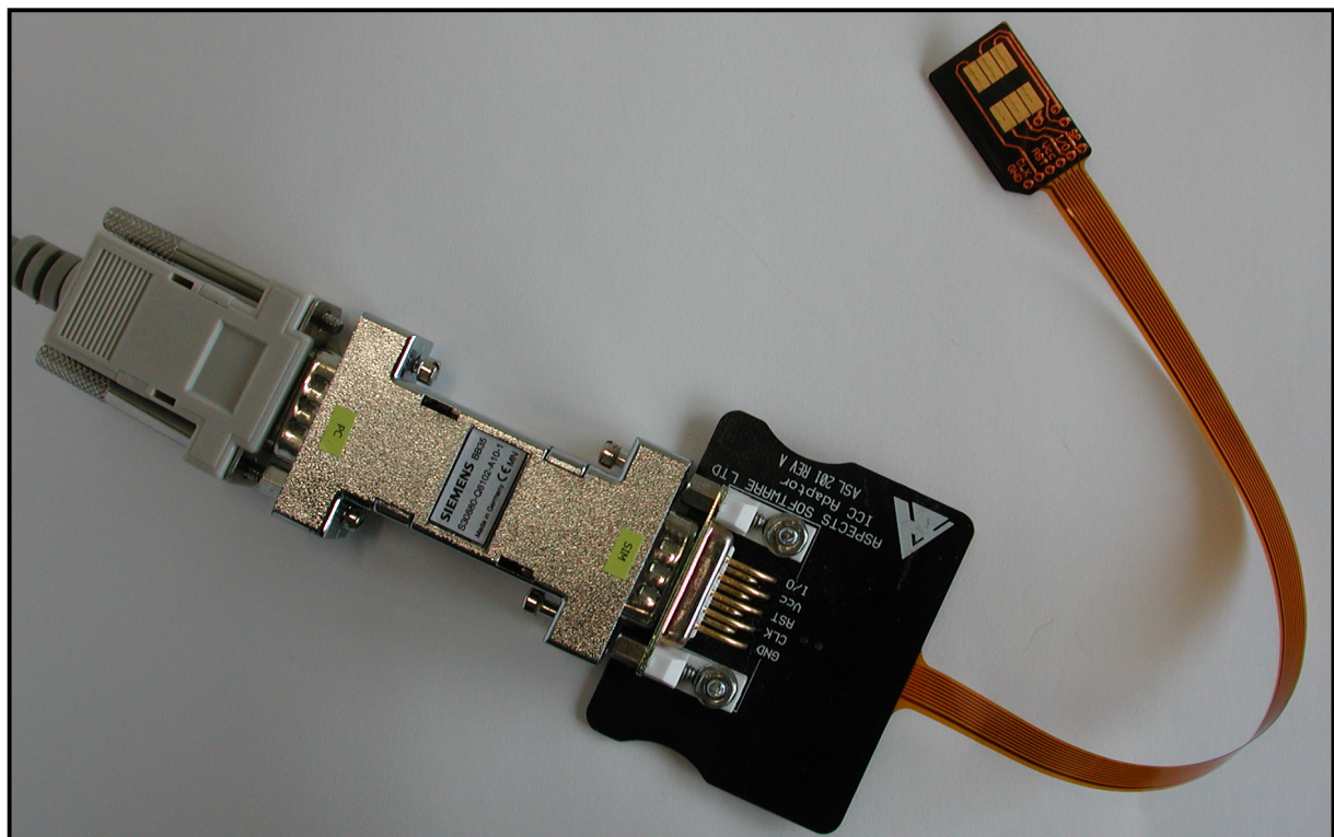
Figure 16: How to connect the supplied cables to the BB35 Bootbox
