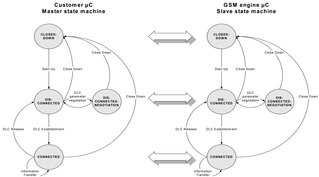
Figure 4: Relationship between the customer μC and the GSM engine μC
