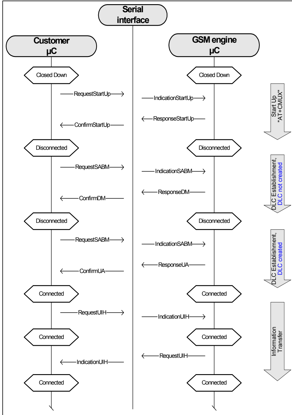
Figure 5: MPI – Startup, DLC establishment and information transfer
