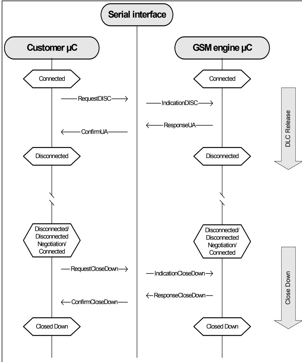
Figure 6: MP - DLC release and close down
