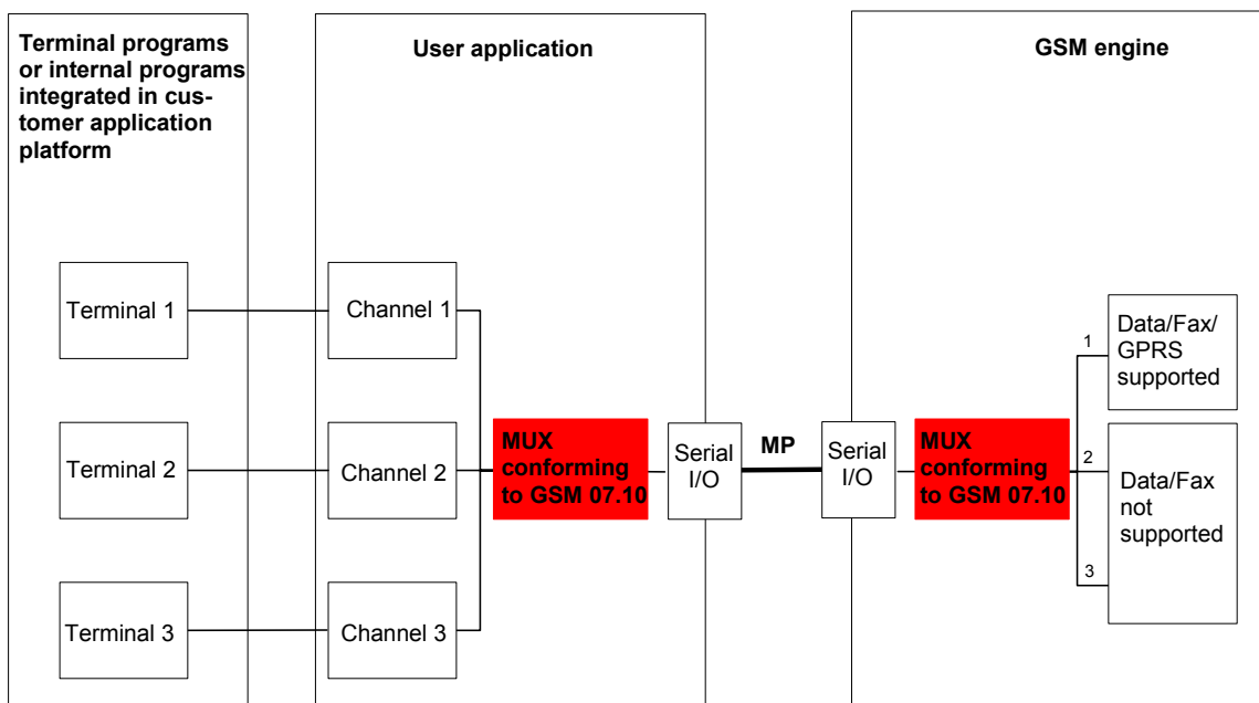
Figure 1: Multiplexer architecture
