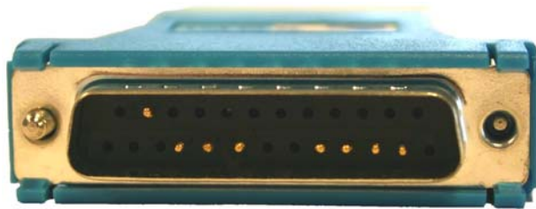
Figure 1: XSPI Adapter Current Model (Pin 24 Ground)
