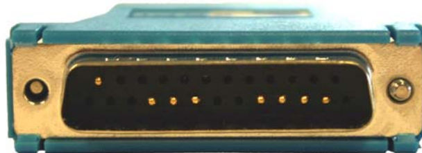
Figure 2: Figure 2: 24-Pin XSPI Adapter Old Model (Pin 25 Ground)
