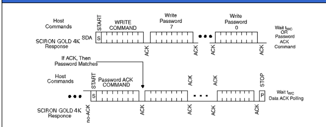
Figure 4. Sector Write Sequence (Password Required)
