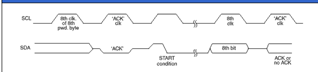
Figure 5. Acknowledge Polling
