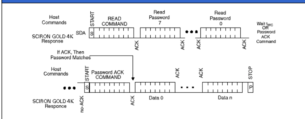
Figure 6. Sector Read Sequence (Password Required)
