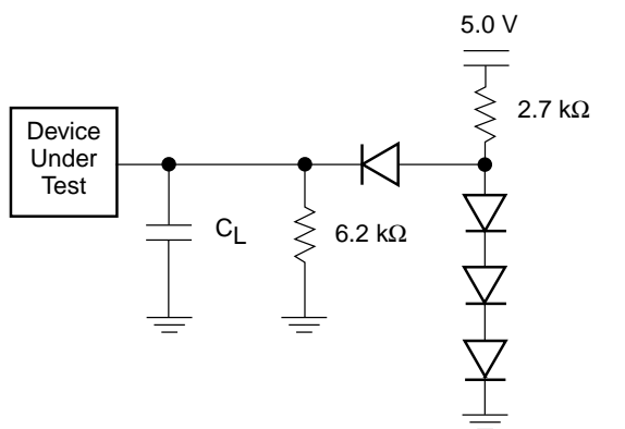
Figure 8. Test Setup
