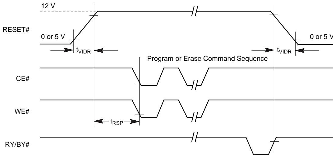
Figure 16. Temporary Sector Group Unprotect Timing Diagram
