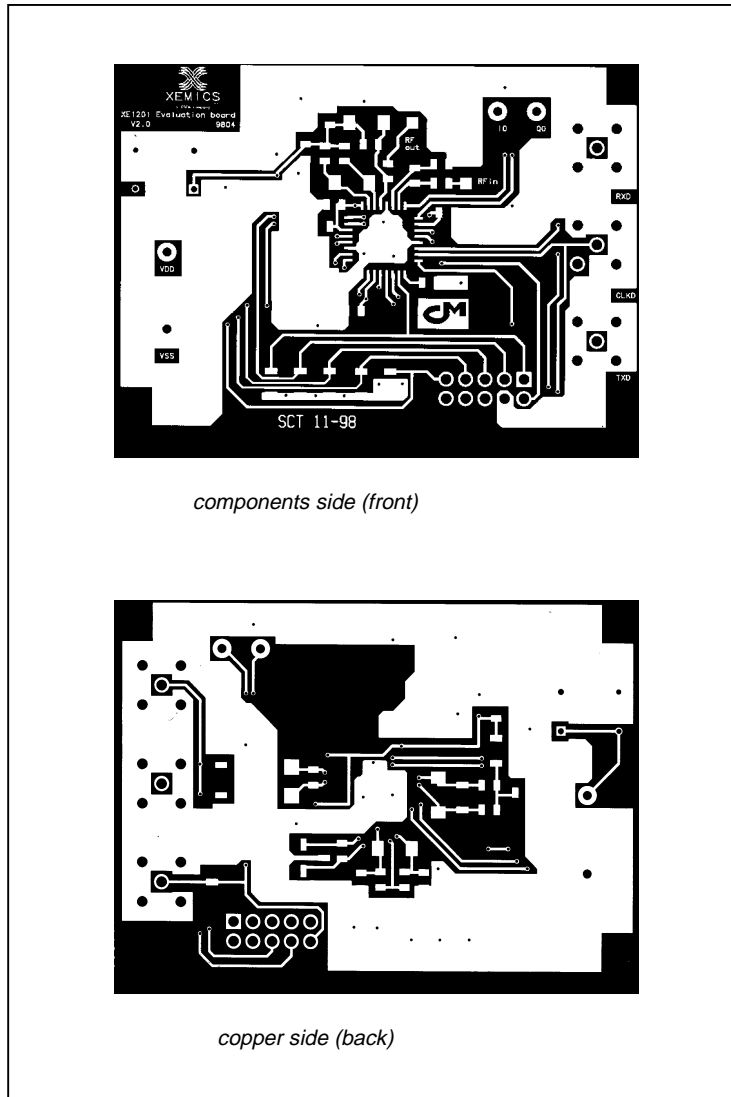
Figure 8: evaluation board layout (not actual scale)
