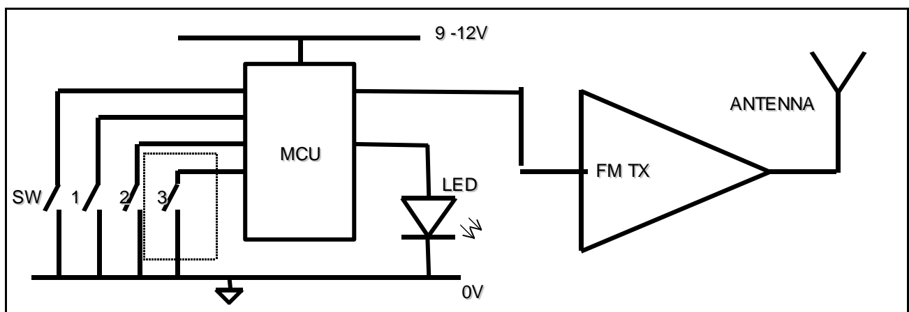
BLOCK DIAGRAM
