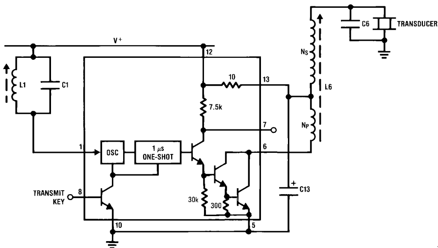
FIGURE 5. Transmitter
