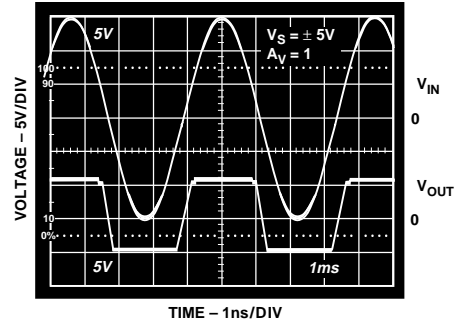
Figure 38. Output Voltage Phase Reversal Behavior
