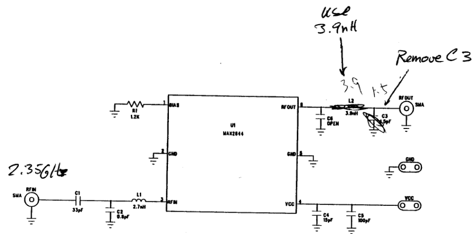
Figure 1. MAX2644 EV Kit Schematic
