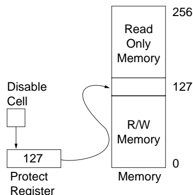
FIGURE 1. Memory Protect Register
